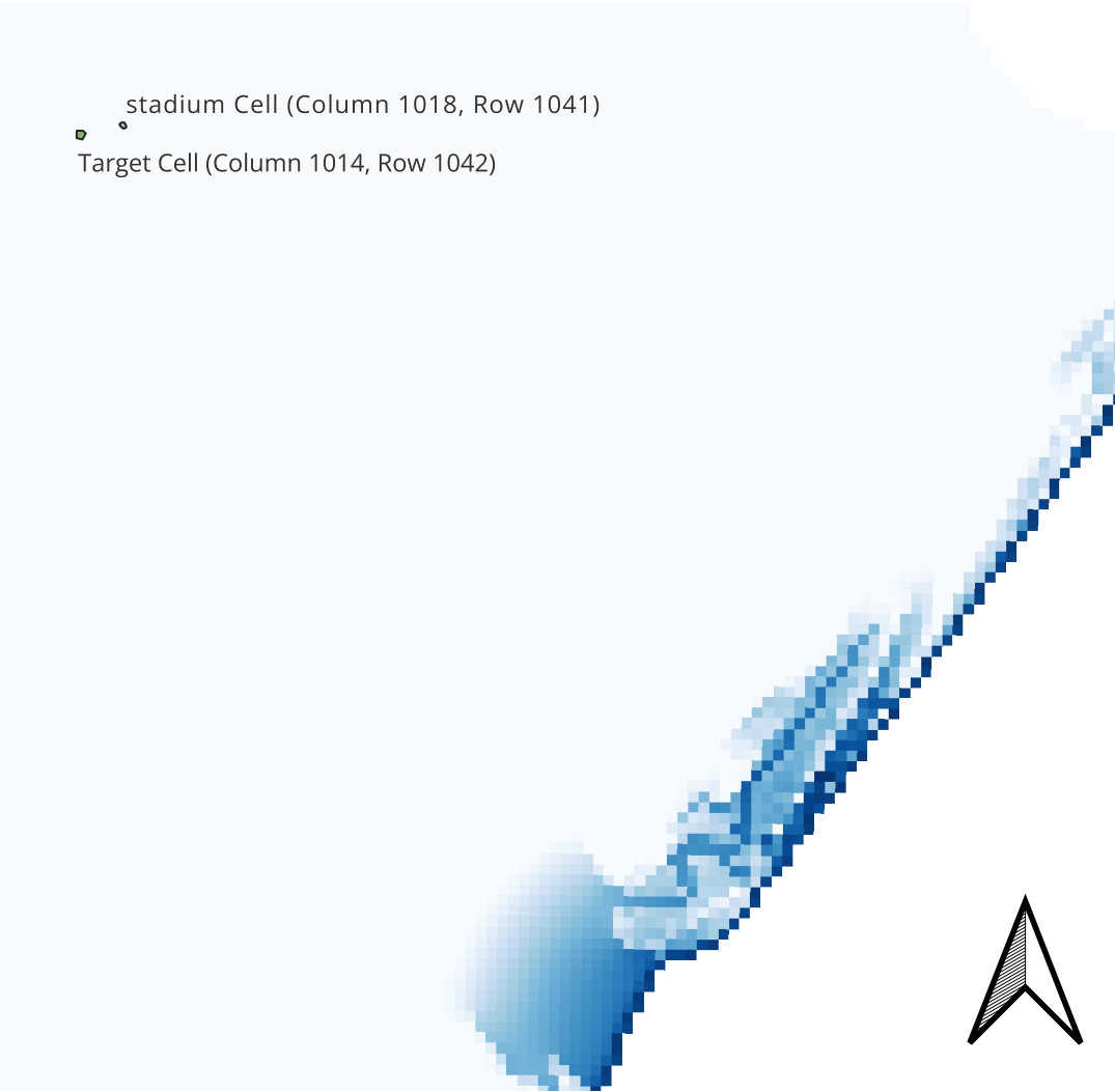
Maximum Water Level - without Rainfall
